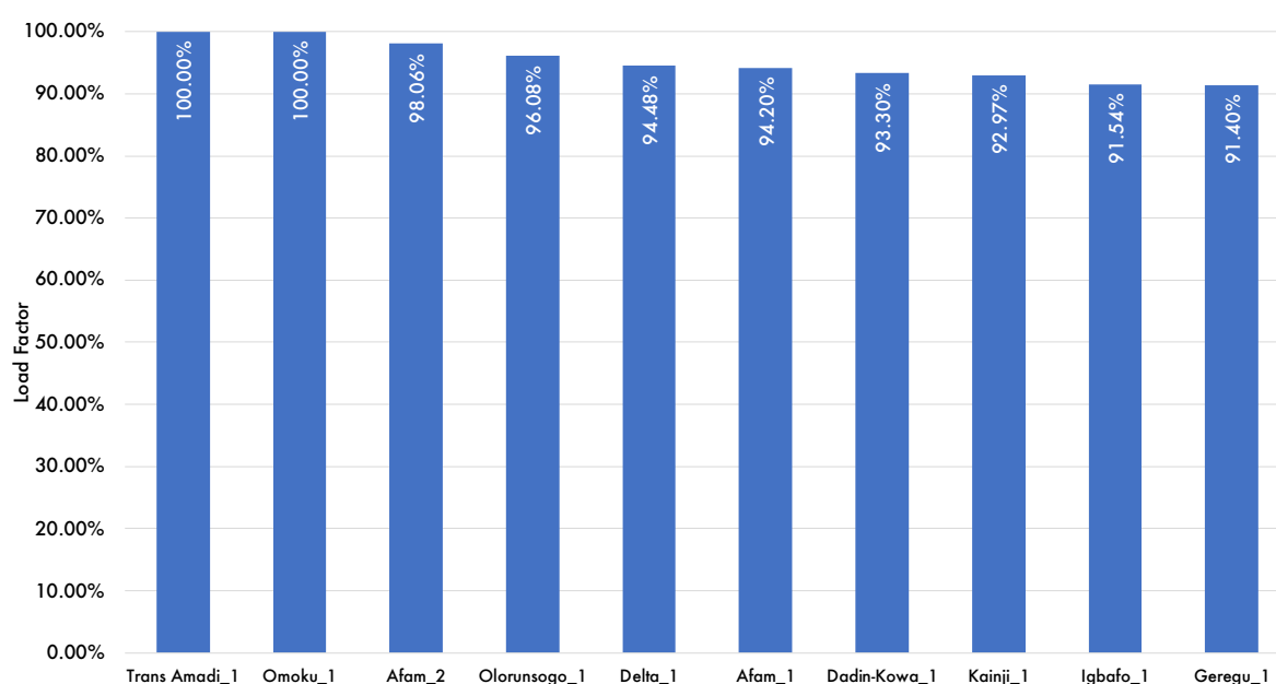
Figure 7.4: Load Factor of Plants with Highest Dispatch Rate (%) in 2024
