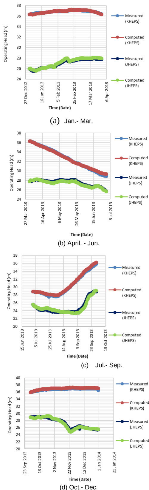
Fig. 2: Comparison of Observed Head with Computed Head for the Cascade KHEPS and JHEPS in 2013
