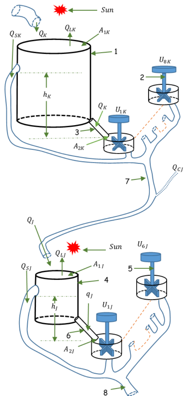
Fig. 1: Schematic Representation of Kainji-Jebba Hydroelectric Power Stations
